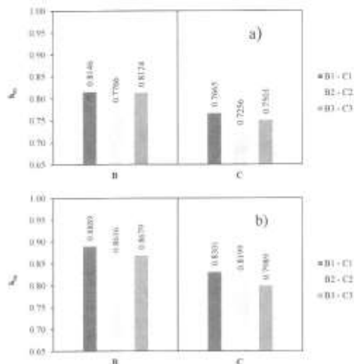
Fig. 10. Comparisons of k_m coefficient for the two series. a) low pressure; b) high pressure.
