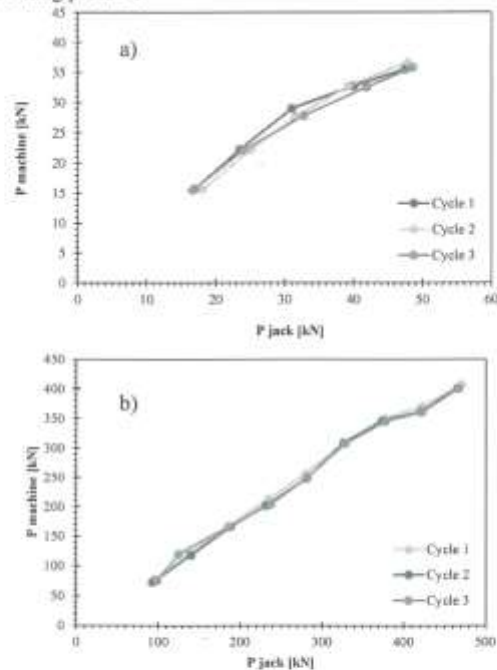
Fig. 4. Results for specimen B1. a) Low pressure; b) High pressure.
