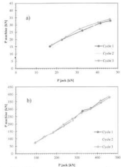
Fig. 6. Results for specimen C1. a) Low pressure; b) High pressure.
