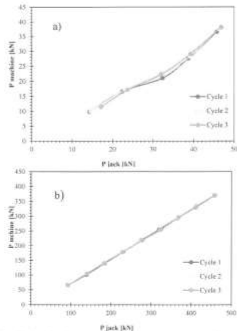
Fig. 7. Results for specimen C3. a) Low pressure; b) High pressure.
