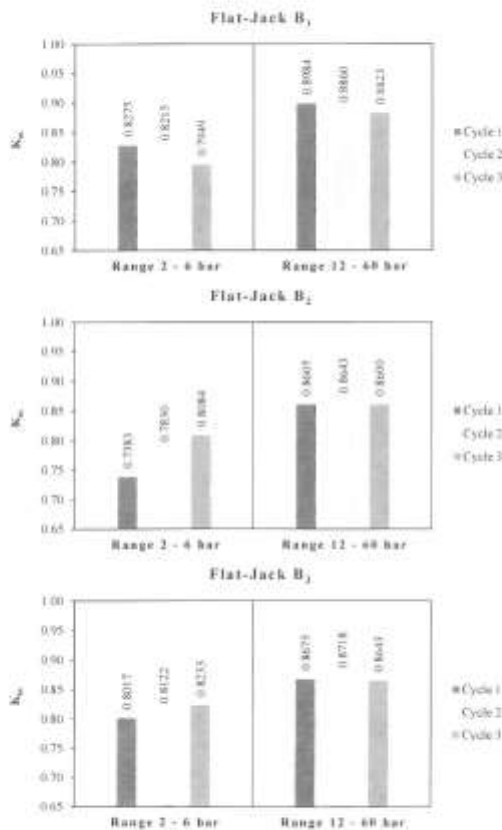
Fig. 8. k_m coefficient for the B-series of flat jacks.
