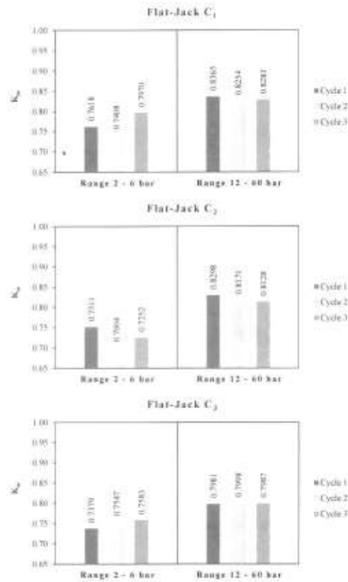
Fig. 9. k_m coefficient for the C-series of flat jacks.
