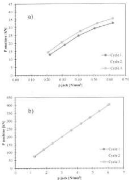
Fig. 5. Results for specimen B2. a) Low pressure; b) High pressure.
