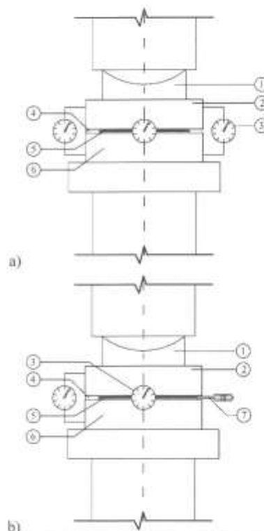
Fig. 2. Test set-up. a) Front view; b) Lateral view.
